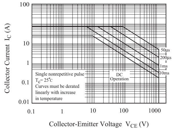
Fig 14. SOA Characteristics
