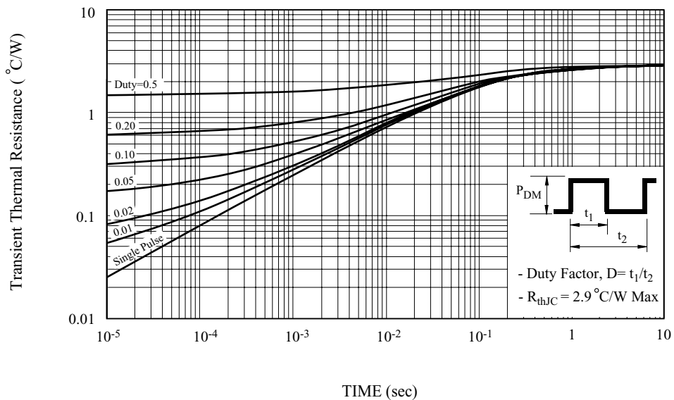
Fig10. Transient Thermal Response Curve
