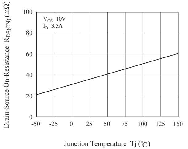
Fig4. R_{DS(ON)} - T_j
